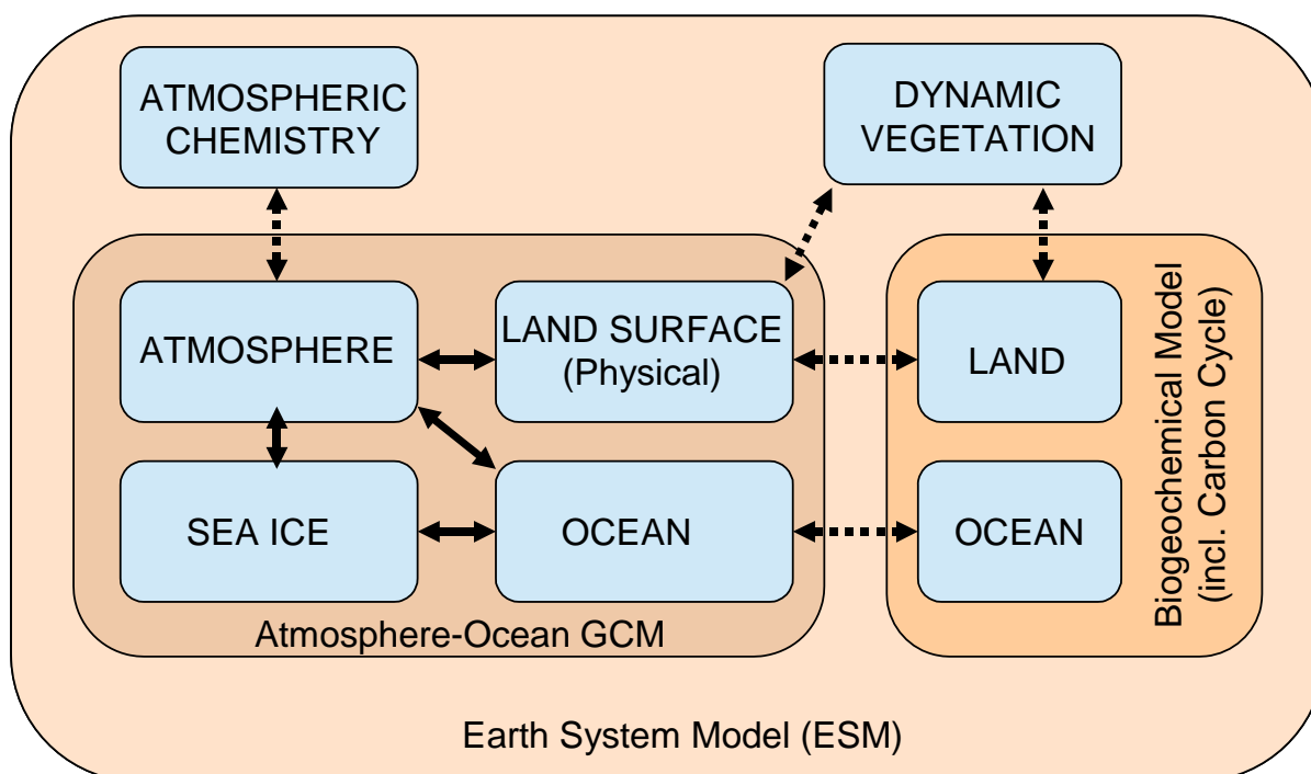
Figure 3.1. The component models that make up an AOGCM and a typical ESM used for climate simulations. Solid arrows represent flow of energy, water, and (in the case of an ESM) GHGs and other atmospheric constituents between component models. Dashed arrows represent the exchange of information within the extended Land, Ocean, and Atmosphere models that make up the ESM. Biogeochemical cycle models include the Carbon Cycle, Nitrogen Cycle, and processes in vegetation, soils, and the upper ocean that model the sources, sinks, and exchange of carbon dioxide, methane, nitrous oxide, and other important GHGs.
